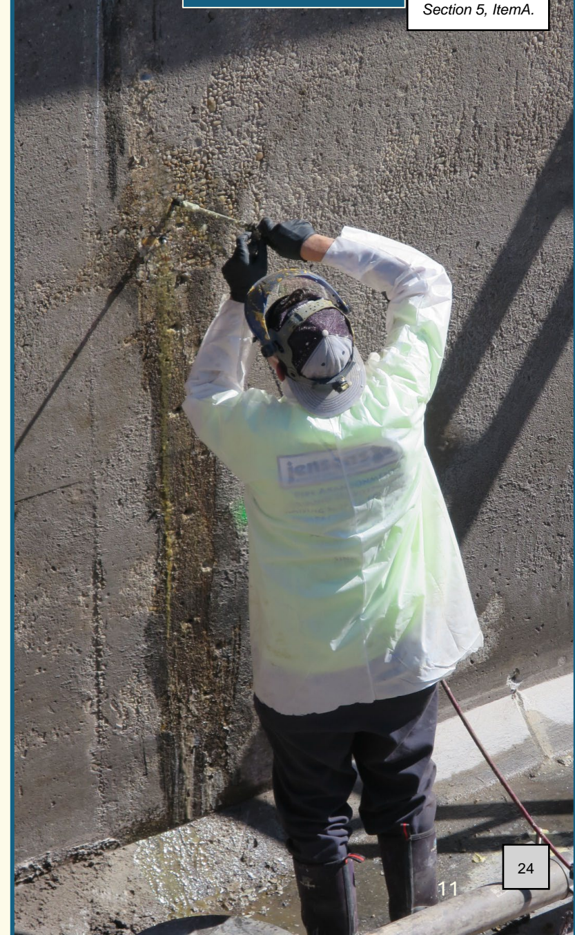
Crack Repair
